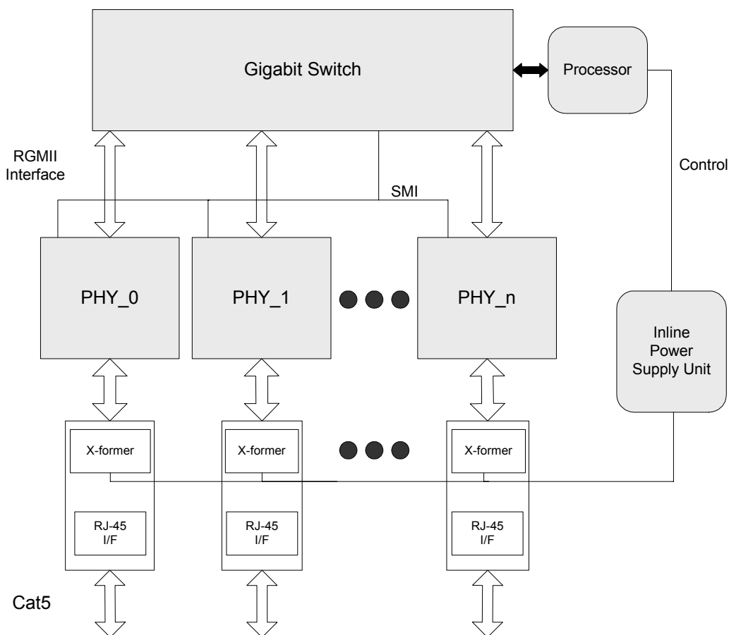
Figure 7. Inline Powered Ethernet Switch Diagram
