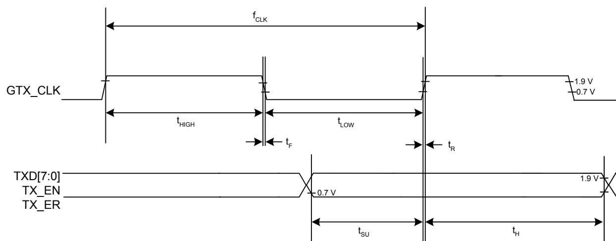
Figure 22. GMII Transmit Timing
